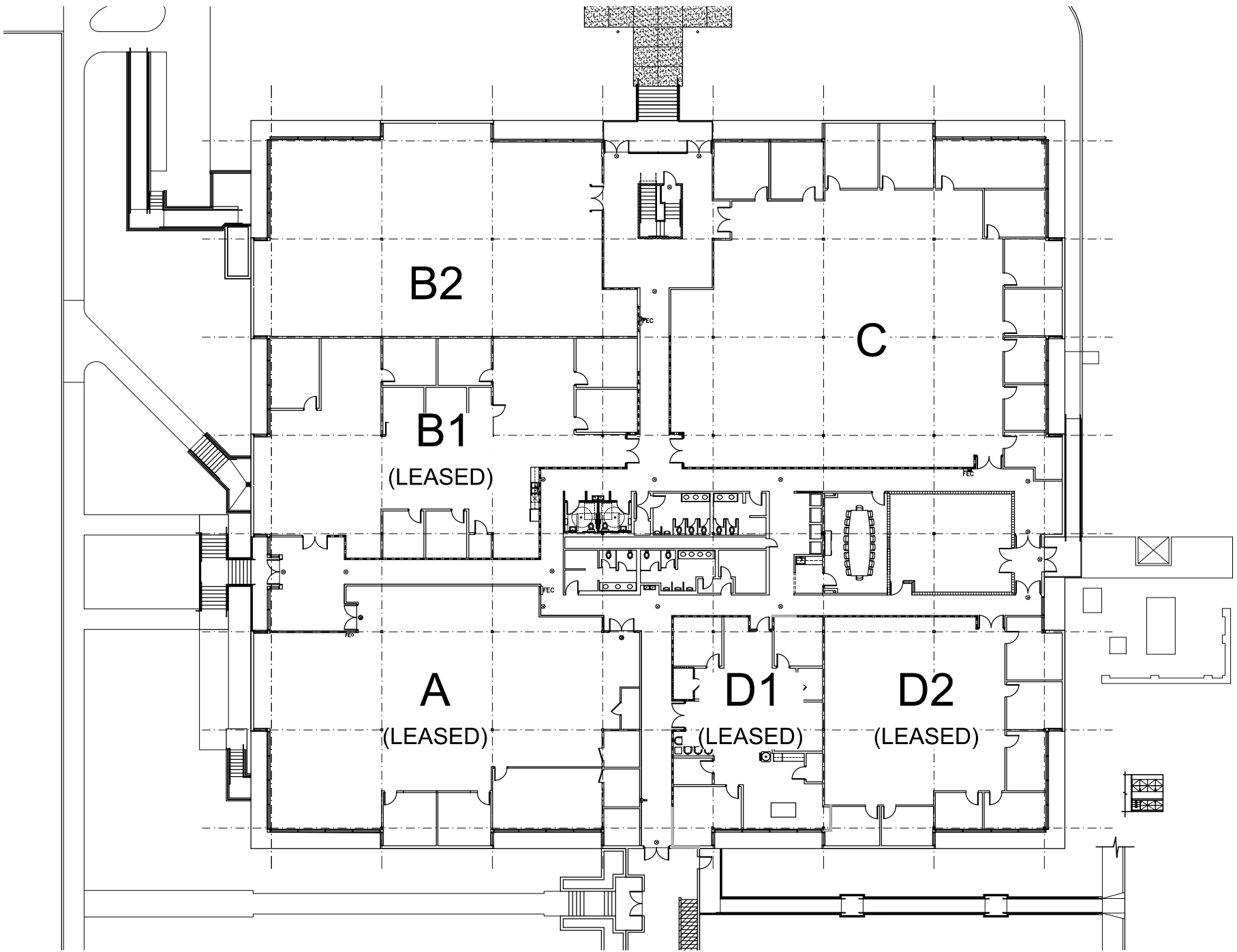
5021 TECHNOLOGY DRIVE FIRST FLOOR TENANT SPACES SCALE: 1/32" = 1'-0"
